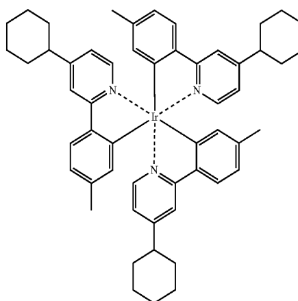
Compound 17
