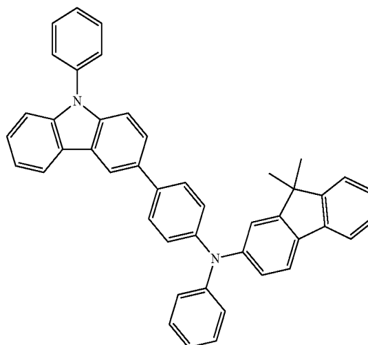
HT2
