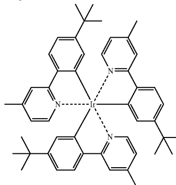
Compound A
