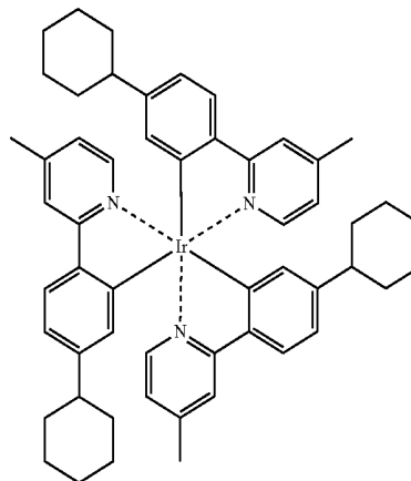
Compound A
